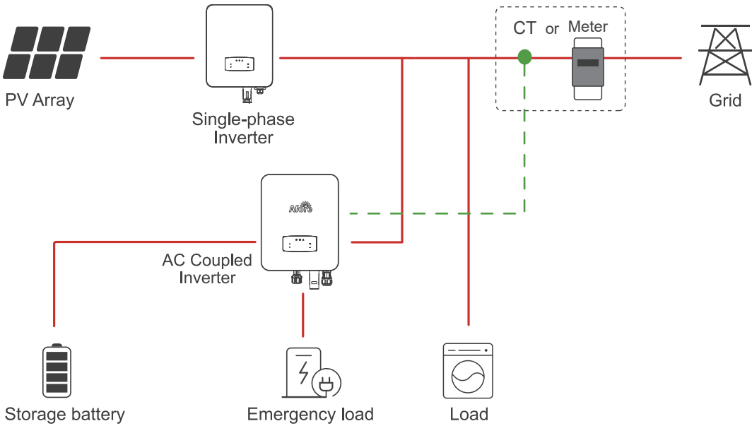
Single Phase AC Coupled (Retro Fit)
