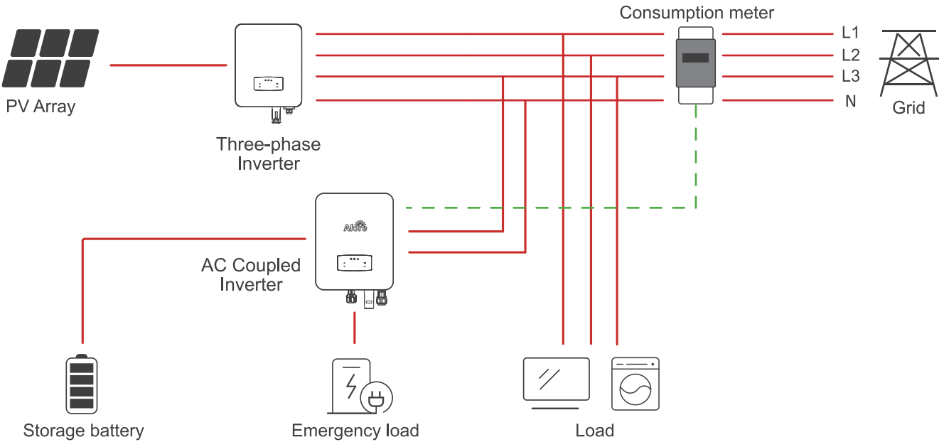
Three Phase AC Coupled (Retro Fit)
